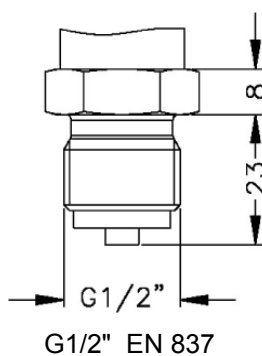
Installation dimensions
