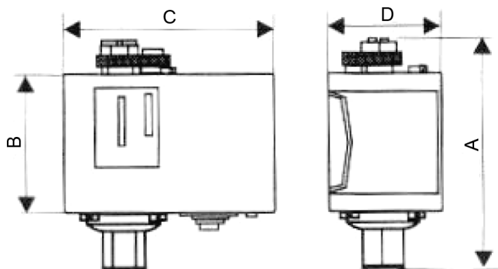
Female threaded connection 1/4G
