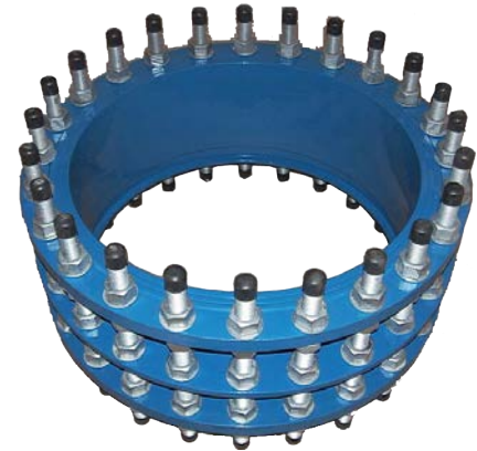
Epoxy coated body according to EN 14901 RAL 5015, 250 µm thickness (WRAS QUALITY)
